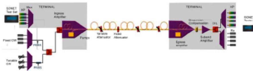
Figure 1. Set-up of the emulated link
