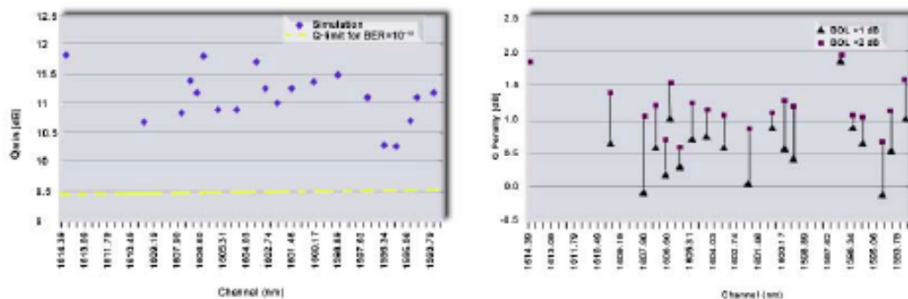
Figure 4: a) BOL Q-performance; b) Q-penalty with respect to baseline in scenario 4
