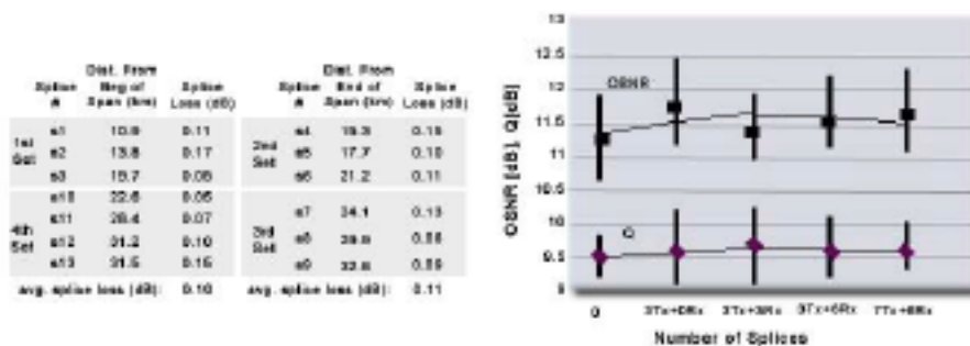
Figure 5: Impact on performance of point losses in shore-end sections
