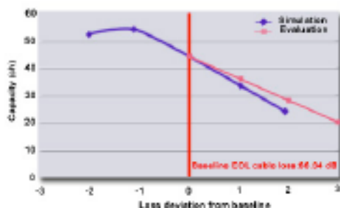
Figure 3. Capacity vs. Loss Deviation from the Baseline
