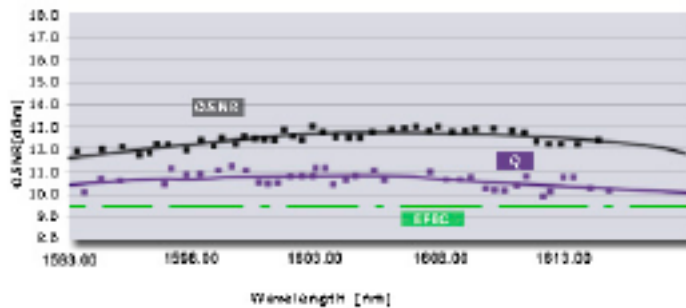
Figure 2. Stability test Average Q and OSNR
